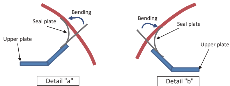
b-1.1) Upper Plate & Seal Plate (detail "a" & "b")
