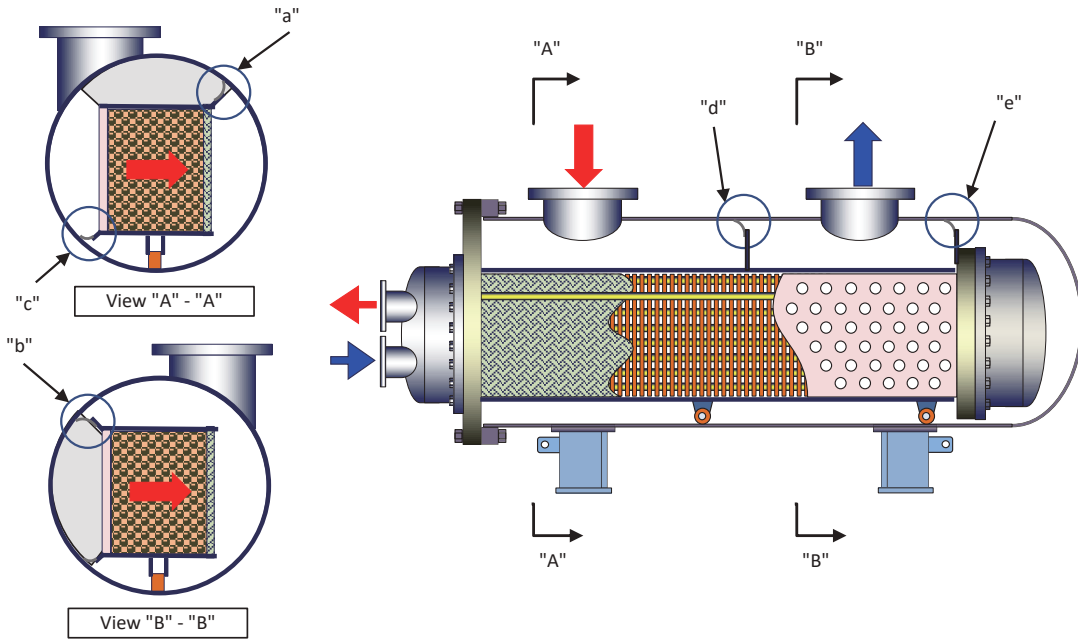
b-1.1) Upper Plate & Seal Plate (detail "a" & "b")
