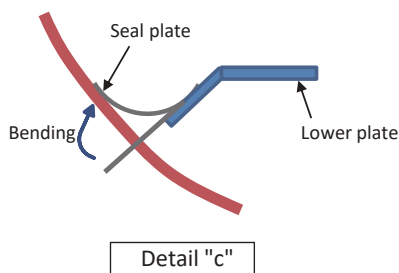
b-1.2) Lower Plate & Seal Plate (detail "c")
