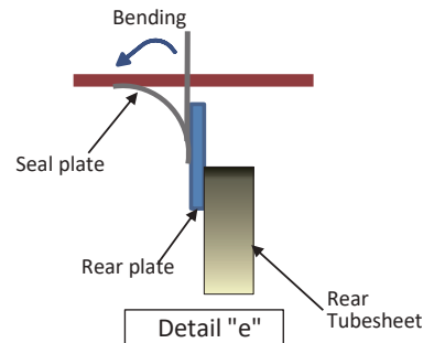
b-1.4) Rear Plate & Seal Plate (detail "e")
